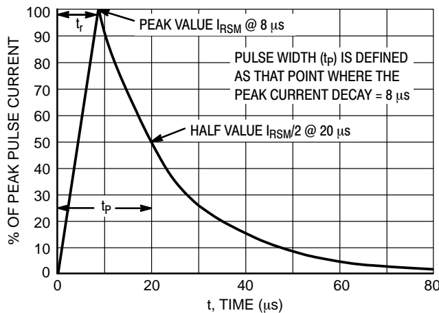
Figure 13. 8 X 20 \mu\text{s} Pulse Waveform
